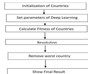
Figure 4: Imperialist Competition algorithm flowchart for calculation of convolution matrix
