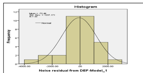
Figure 5: Histogram of rest of the ARIMA model 0,1,1
